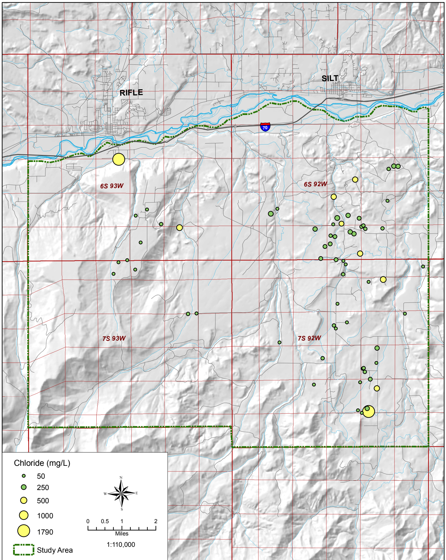
Figure 4.7. Chloride Concentration Distribution in Domestic Wells
