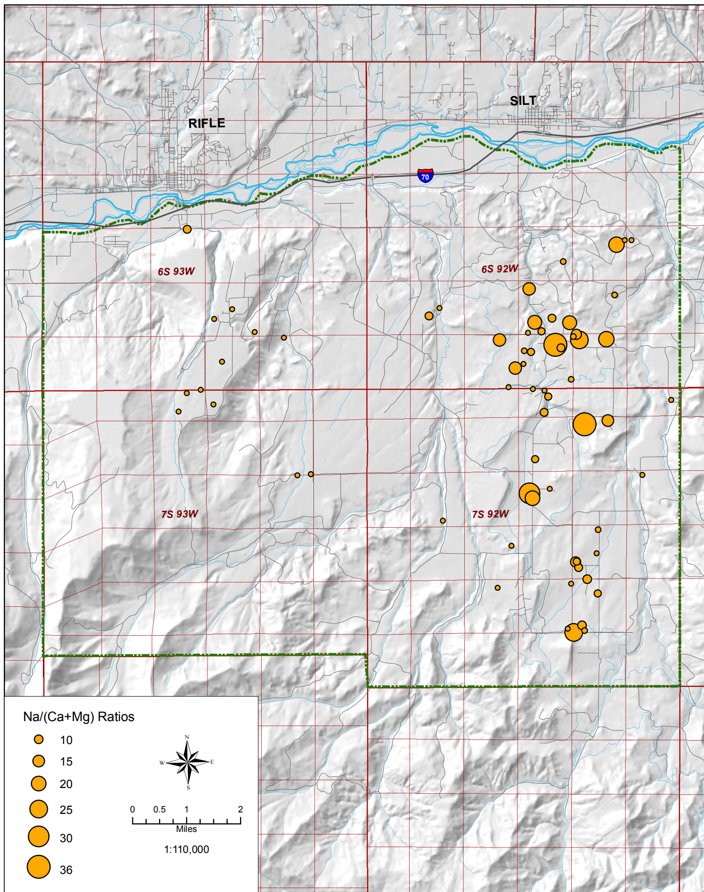
Figure 4.12. Na/(Ca+Mg) Ratios for Domestic Well Samples
