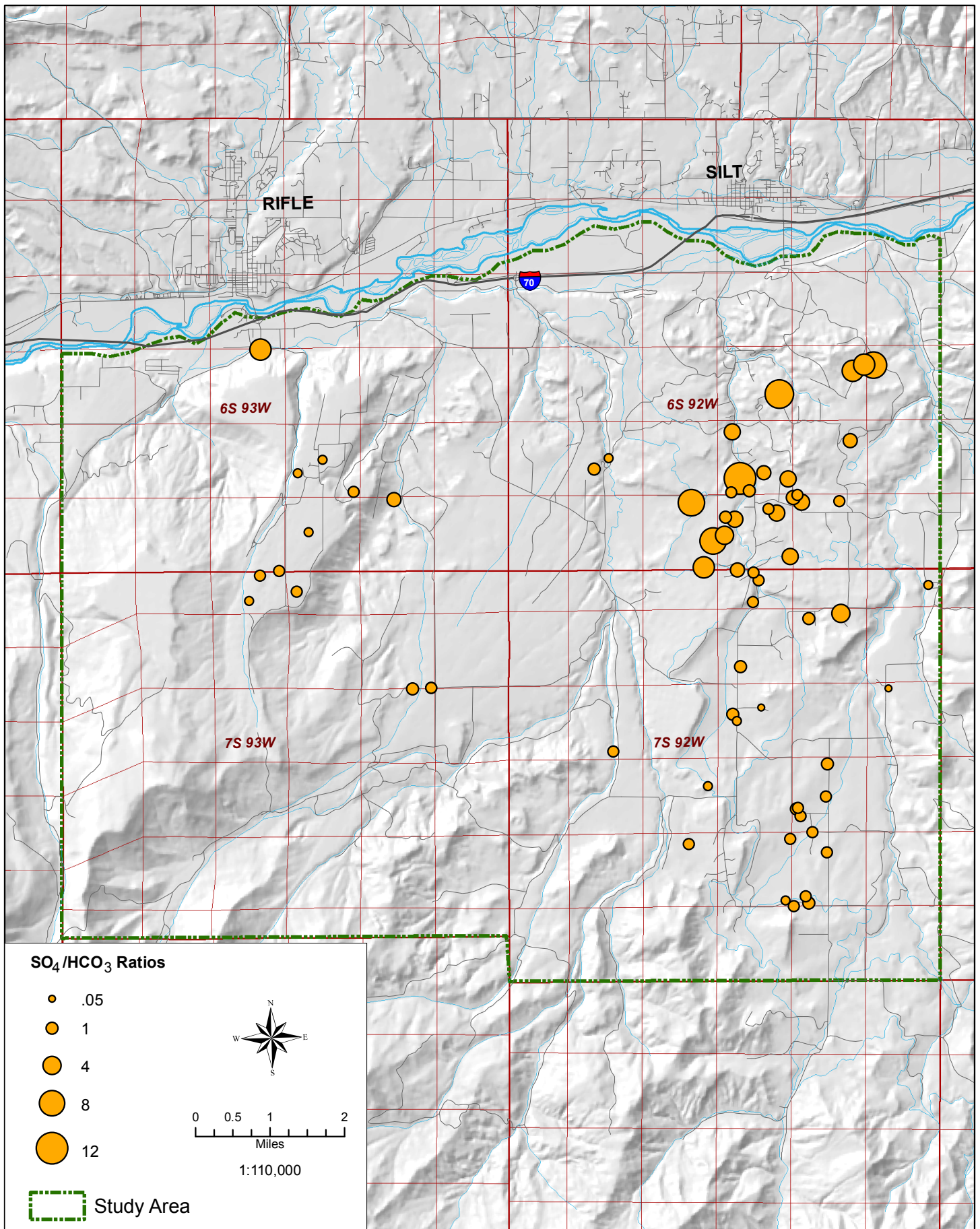
Figure 4.13. \text{SO}_4/\text{HCO}_3 Ratios for Domestic Well Samples
