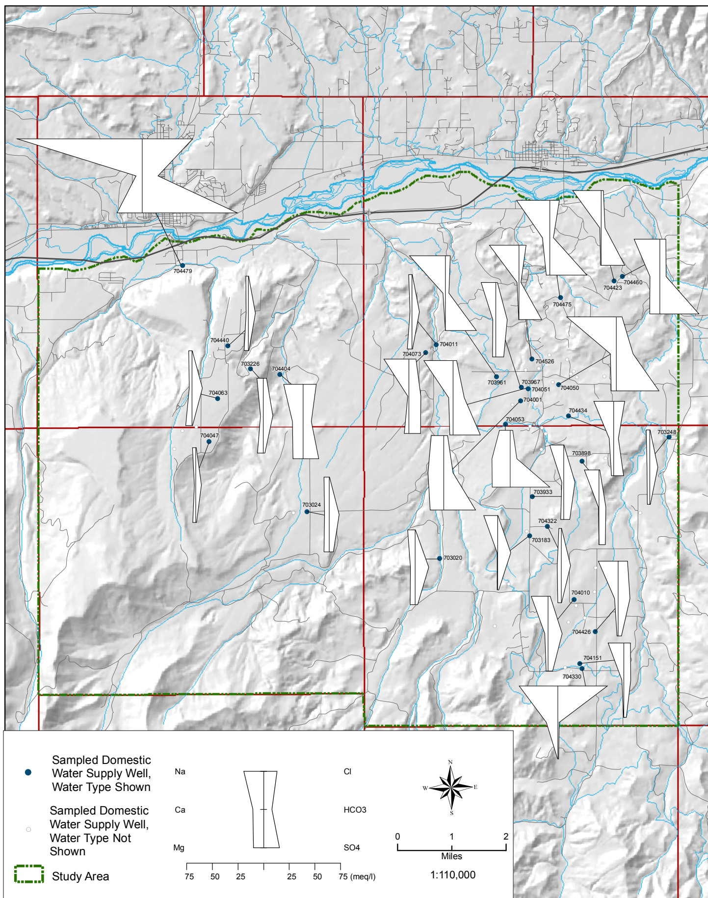
Figure 4.14. Distribution of Water Types for Selected Domestic Wells Using Stiff Plots
