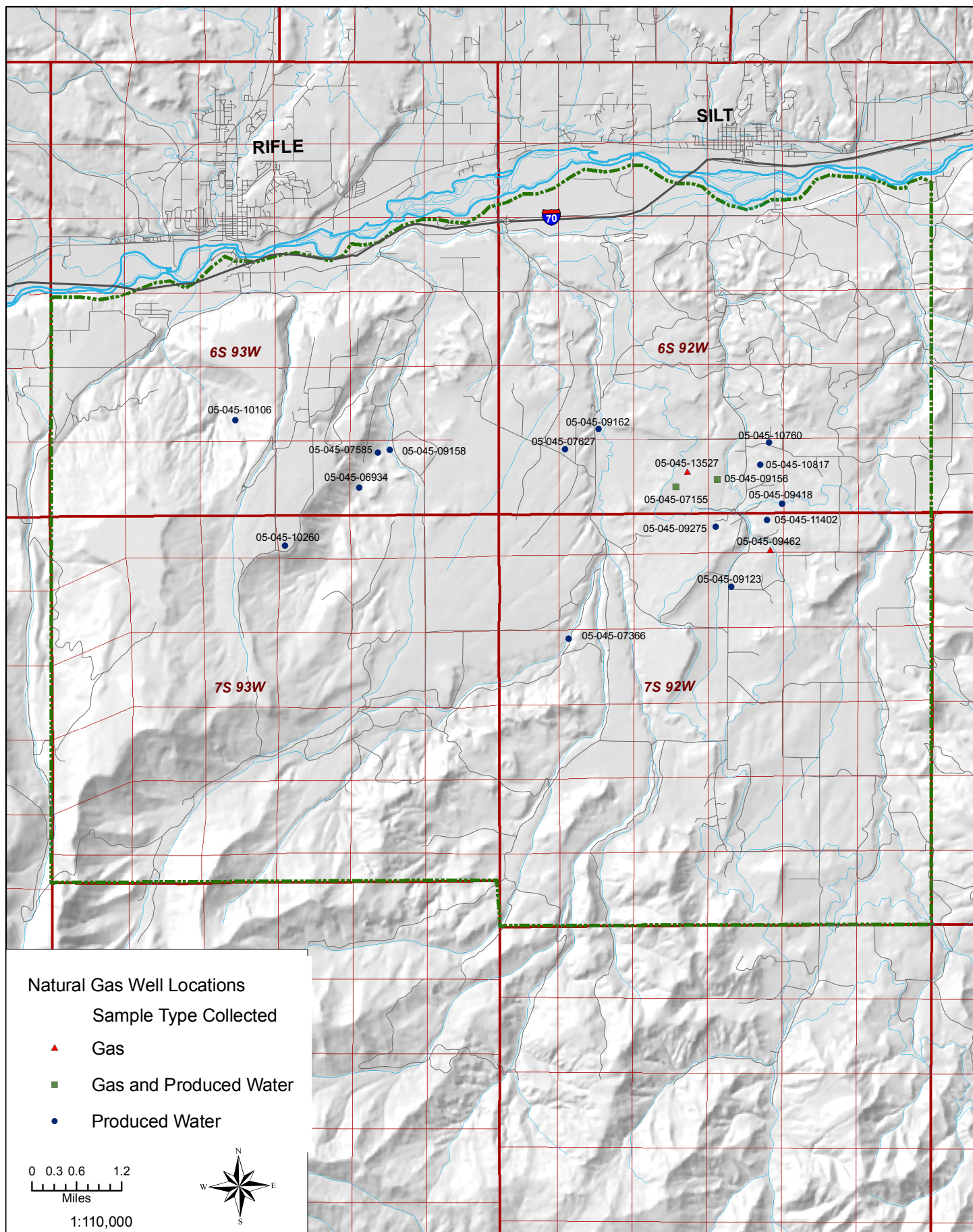
Figure 4.2. Location of Natural Gas Well Samples
